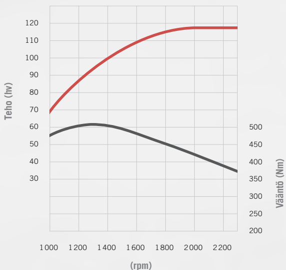
Farmall 120 C
